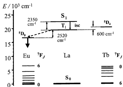
Figure 6. Schematic energy diagram for [\text{Ln}(\text{L}^{12})_3]^{3+} complexes. Data for S_1 and T_1 are those of the \text{La}^{\text{III}} complex in the solid state at 77 K (0-phonon transitions).
