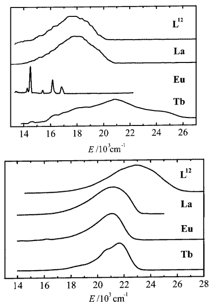
Figure 5. Top: Time-resolved emission spectra of \mathbf{L}^{12} and [\text{Ln}(\mathbf{L}^{12})_3]^{3+} in the solid state at 77 K and recorded with time delays of 0.01 (Eu), 0.1 (Tb) and 10 ms ( \mathbf{L}^{12} , La). Bottom: Emission spectra of [\text{Ln}(\mathbf{L}^{12})_3]^{3+} and \mathbf{L}^{12} ( 10^{-3} M in MeCN at 293 K).
